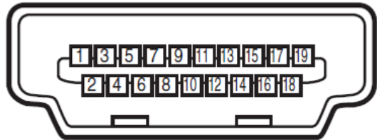
HDMI(19 pin Type A)
